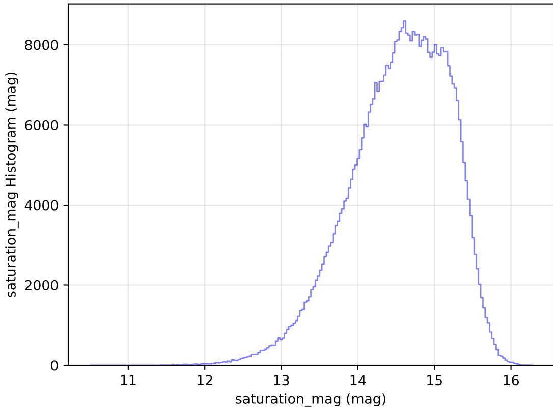
noroll_mjdp120_v3.4_10yrs All sky r band: saturation_mag Histogram
