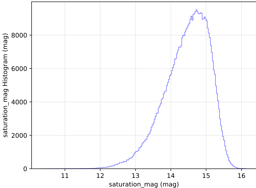
noroll_mjdp120_v3.4_10yrs All sky i band: saturation_mag Histogram
