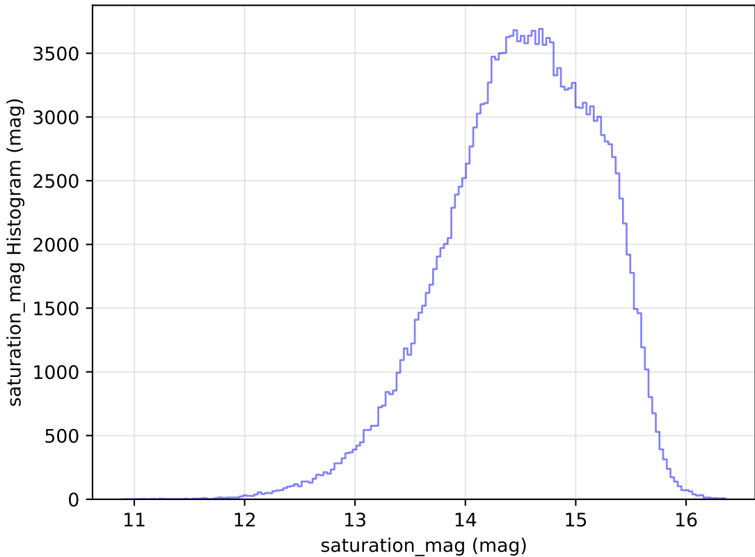
noroll_mjdp120_v3.4_10yrs All sky g band: saturation_mag Histogram
