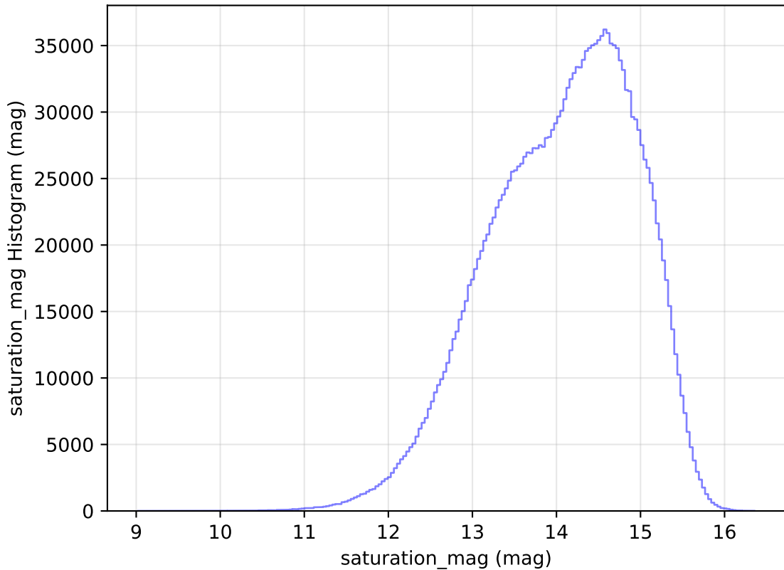
noroll_mjdp120_v3.4_10yrs All sky all bands: saturation_mag Histogram
