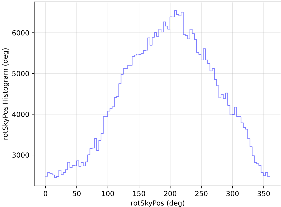
noroll_mjdp120_v3.4_10yrs WFD z band: rotSkyPos Histogram
