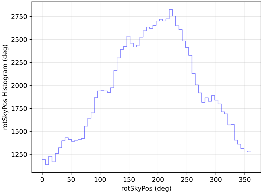
noroll_mjdp120_v3.4_10yrs WFD u band: rotSkyPos Histogram
