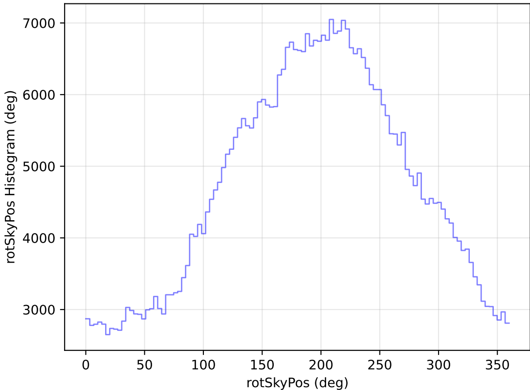
noroll_mjdp120_v3.4_10yrs WFD i band: rotSkyPos Histogram
