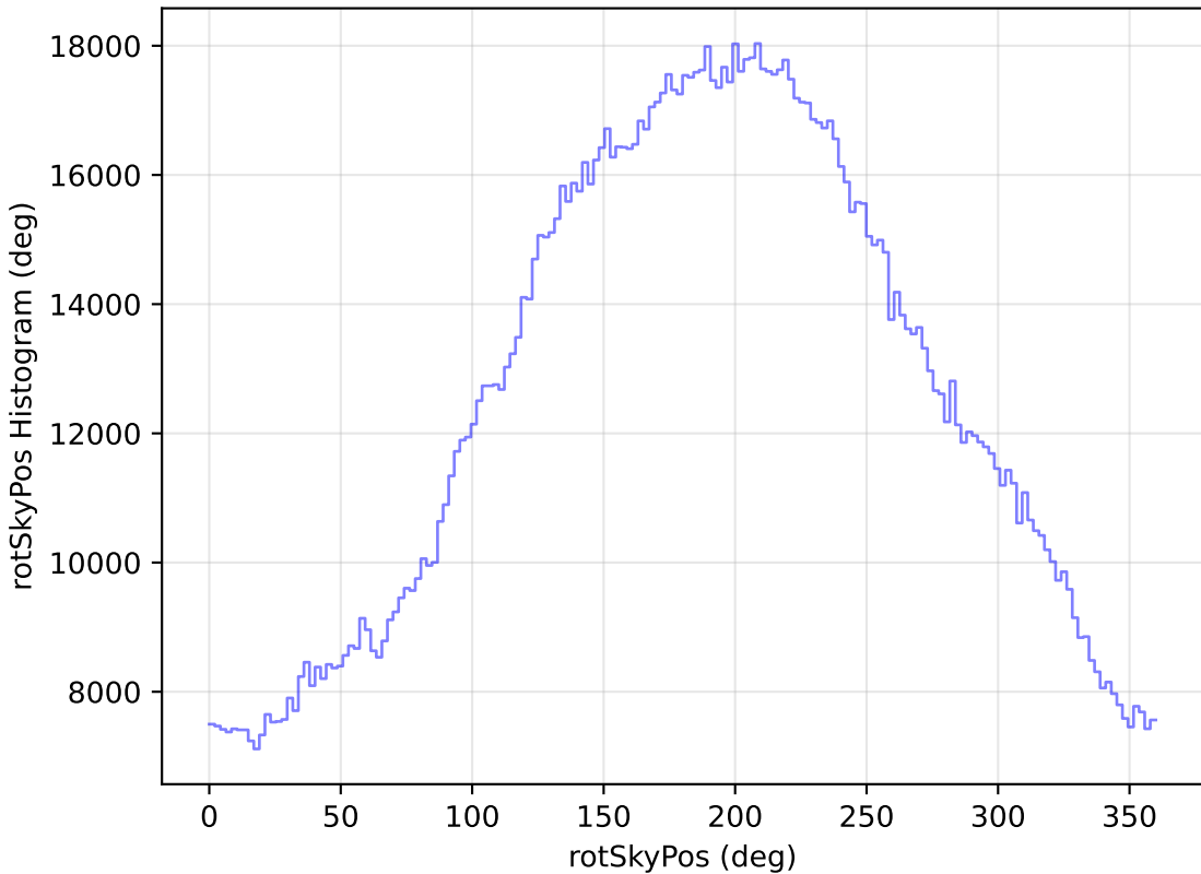
noroll_mjdp120_v3.4_10yrs WFD all bands: rotSkyPos Histogram
