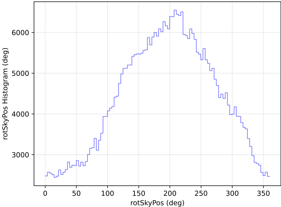
noroll_mjdp120_v3.4_10yrs All sky z band: rotSkyPos Histogram
