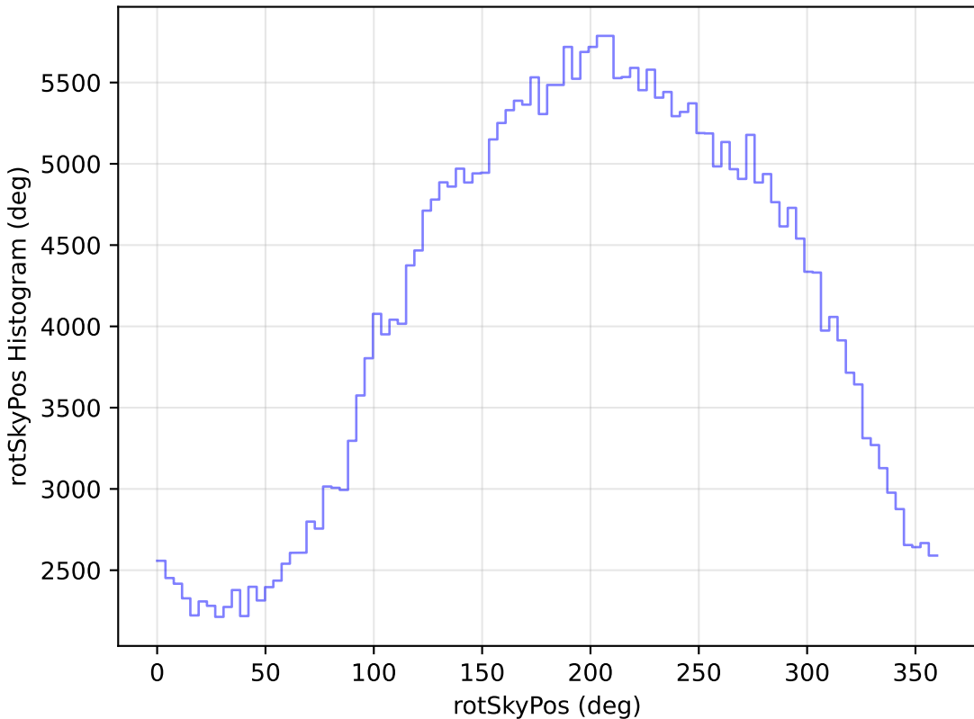
noroll_mjdp120_v3.4_10yrs All sky y band: rotSkyPos Histogram
