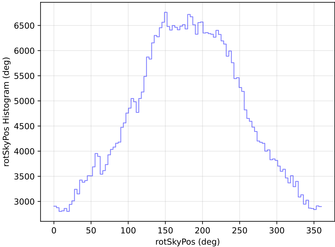
noroll_mjdp120_v3.4_10yrs All sky r band: rotSkyPos Histogram
