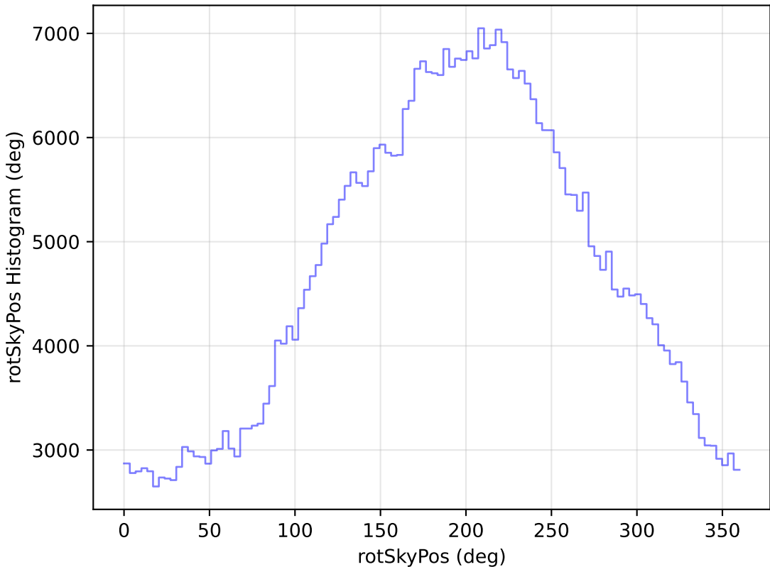
noroll_mjdp120_v3.4_10yrs All sky i band: rotSkyPos Histogram
