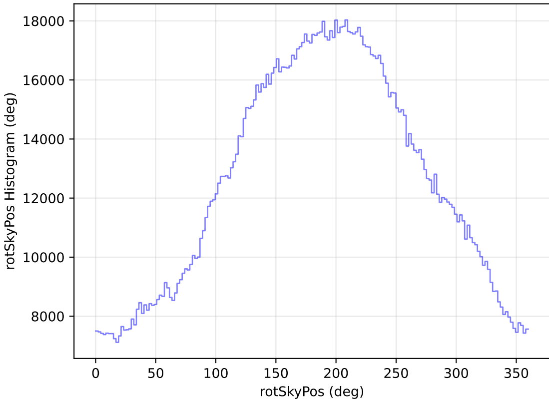
noroll_mjdp120_v3.4_10yrs All sky all bands: rotSkyPos Histogram
