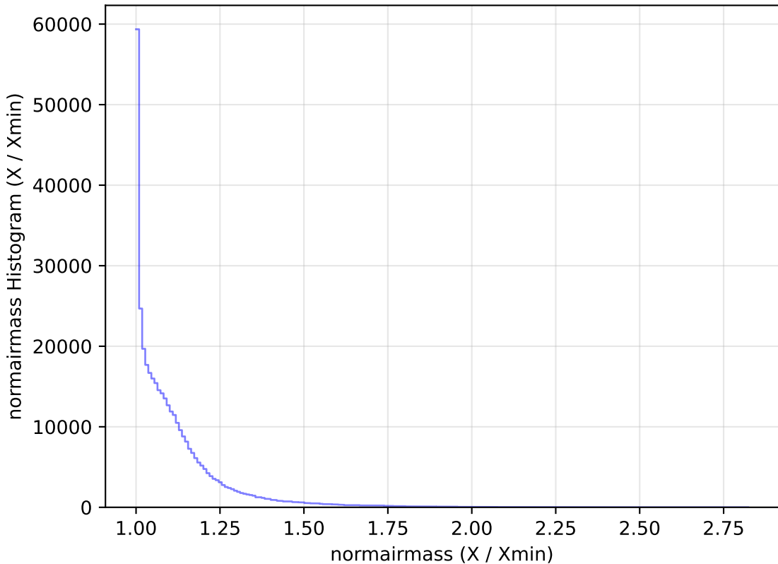
noroll_mjdp120_v3.4_10yrs WFD y band: normairmass Histogram
