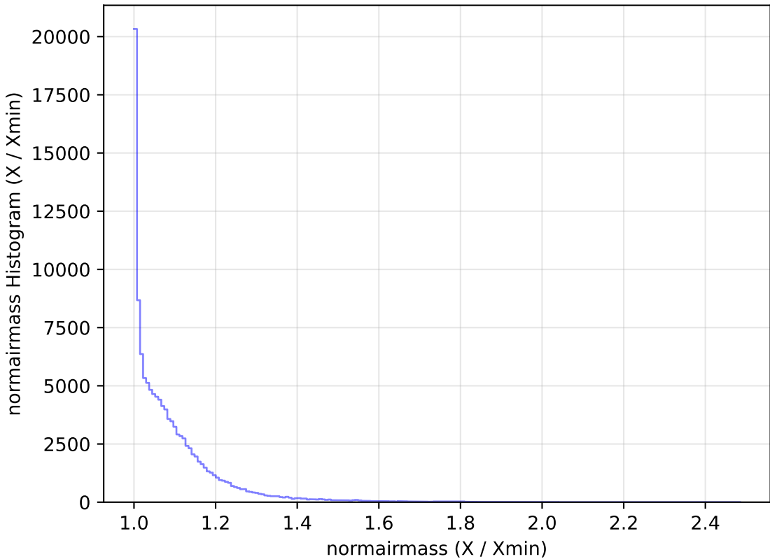
noroll_mjdp120_v3.4_10yrs WFD u band: normairmass Histogram
