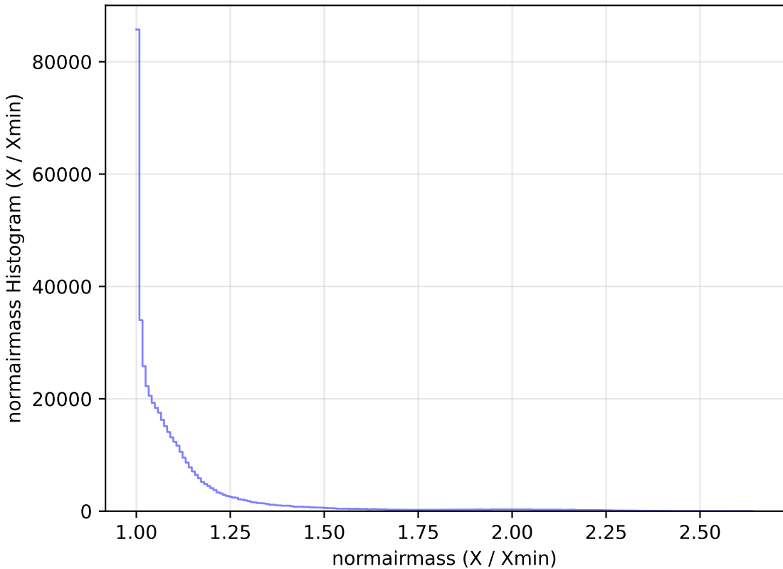
noroll_mjdp120_v3.4_10yrs WFD r band: normairmass Histogram
