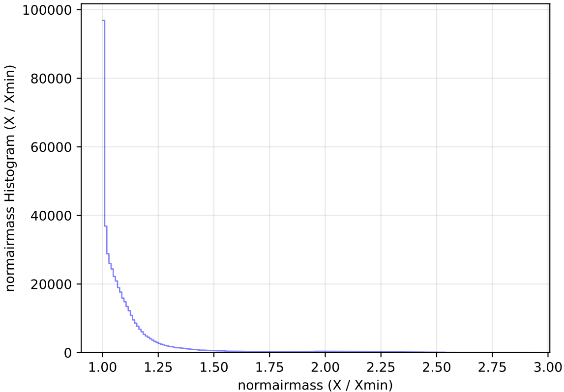
noroll_mjdp120_v3.4_10yrs WFD i band: normairmass Histogram
