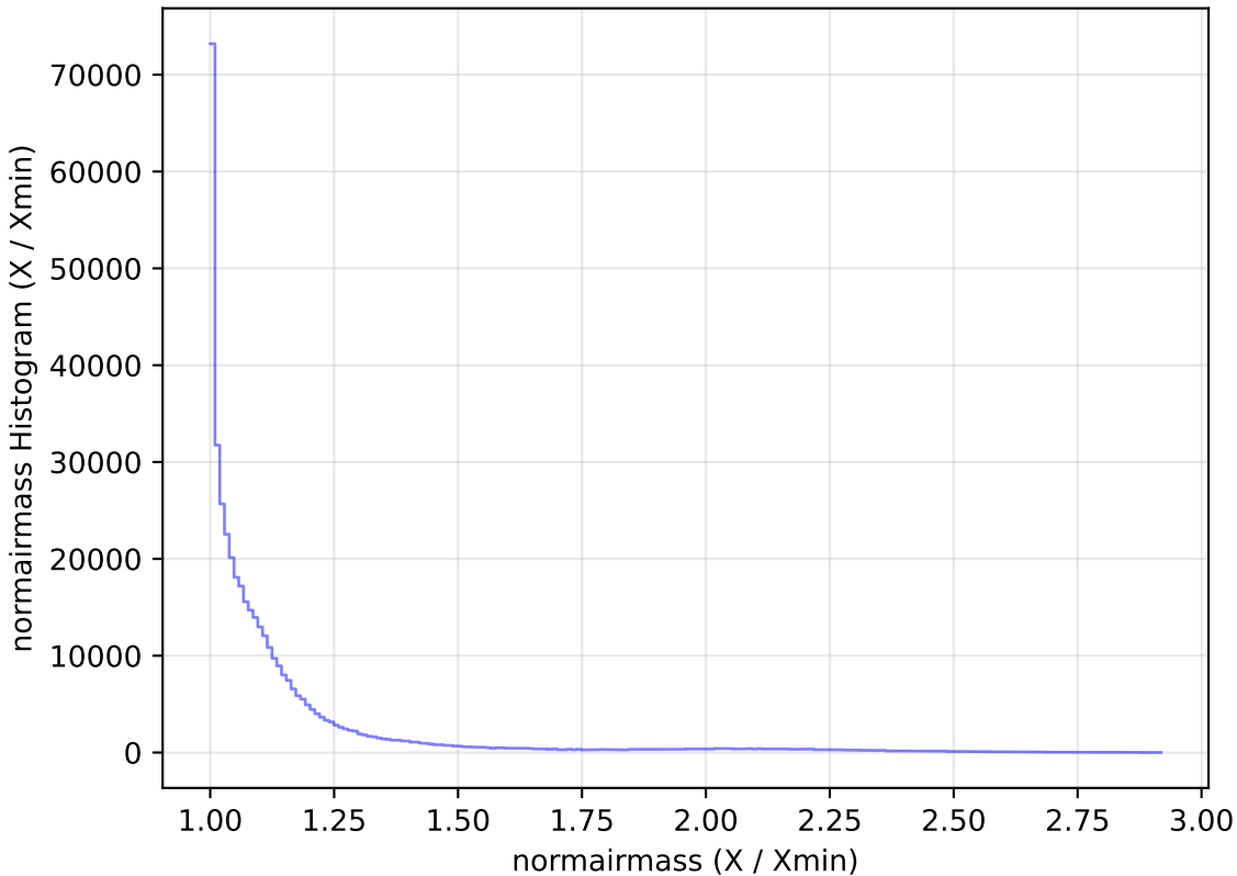
noroll_mjdp120_v3.4_10yrs All sky z band: normairmass Histogram
