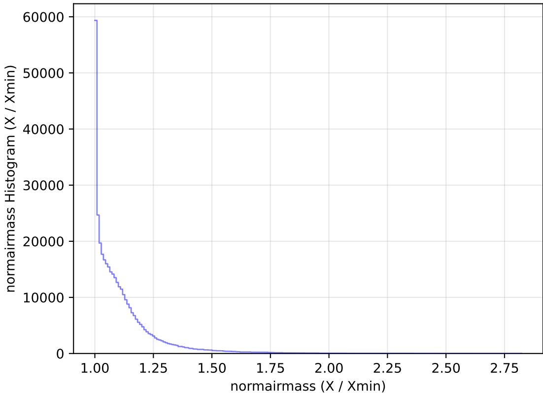
noroll_mjdp120_v3.4_10yrs All sky y band: normairmass Histogram
