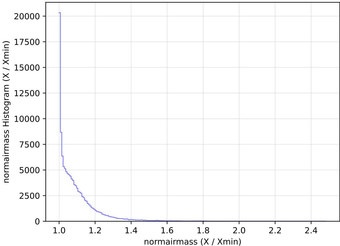
noroll_mjdp120_v3.4_10yrs All sky u band: normairmass Histogram
