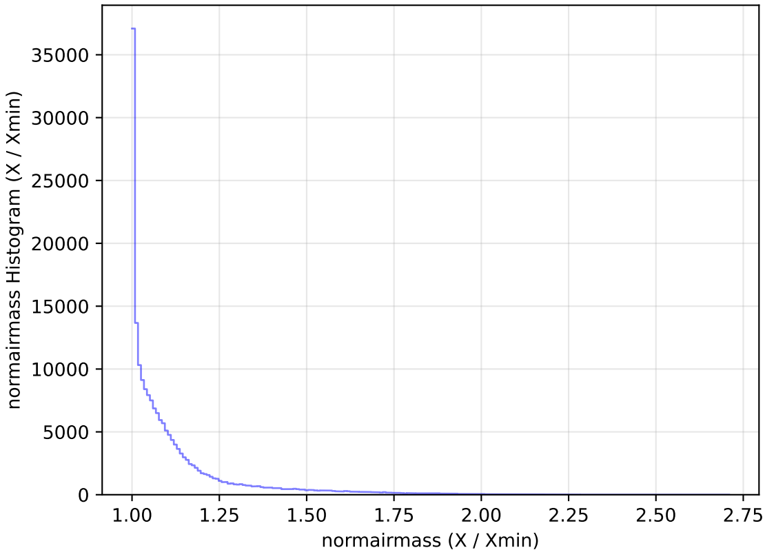
noroll_mjdp120_v3.4_10yrs All sky g band: normairmass Histogram
