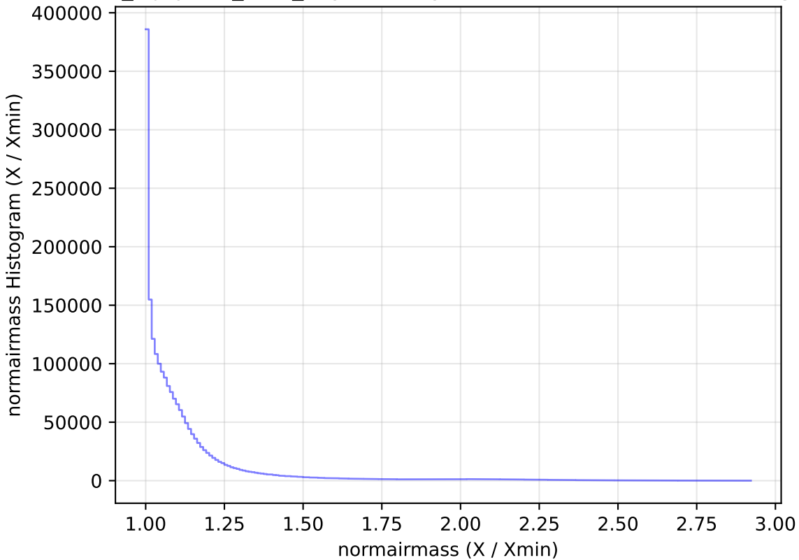
noroll_mjdp120_v3.4_10yrs All sky all bands: normairmass Histogram
