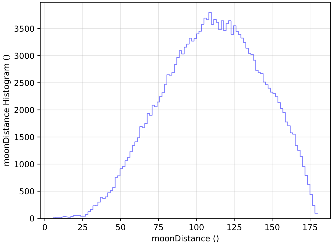
noroll_mjdp120_v3.4_10yrs WFD g band: moonDistance Histogram
