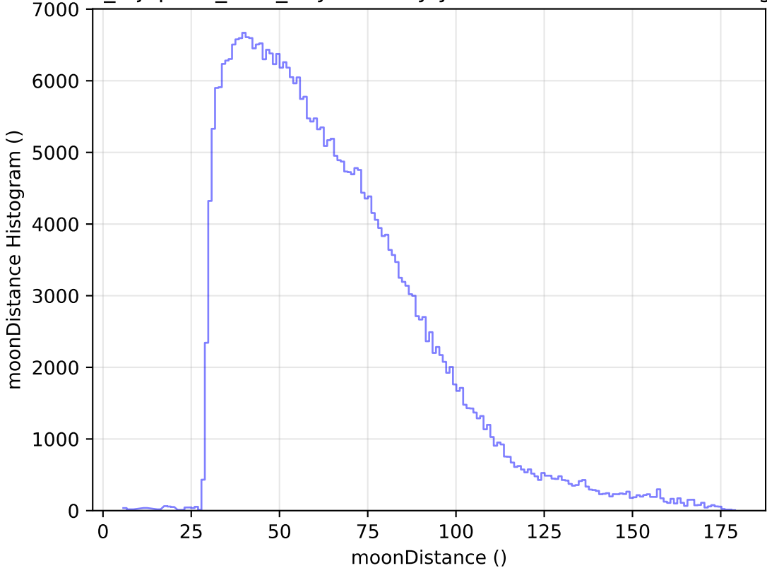
noroll_mjdp120_v3.4_10yrs All sky y band: moonDistance Histogram
