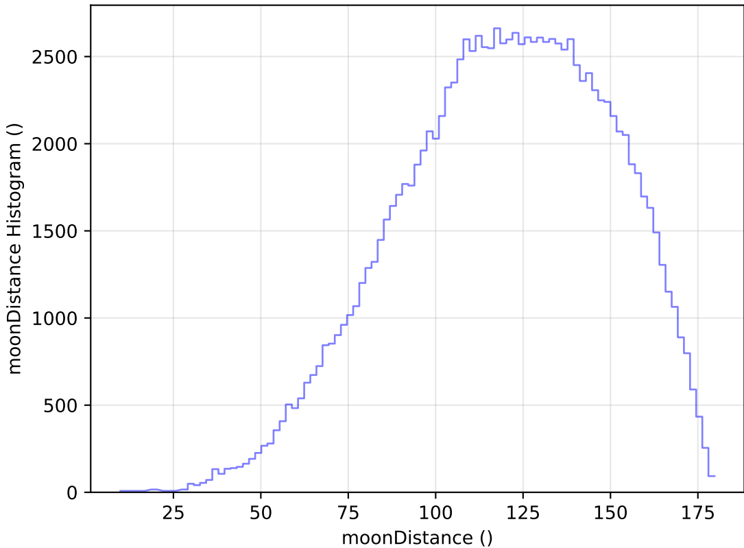
noroll_mjdp120_v3.4_10yrs All sky u band: moonDistance Histogram
