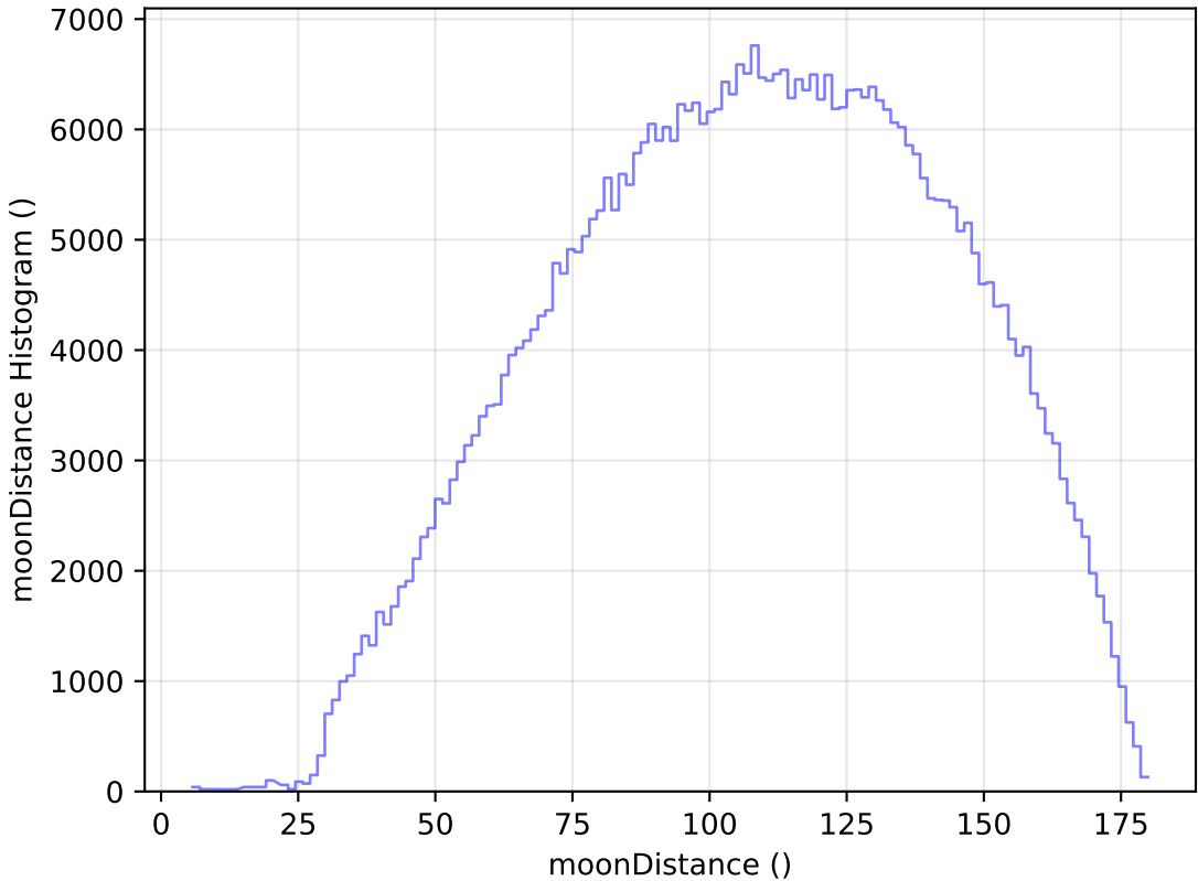
noroll_mjdp120_v3.4_10yrs All sky r band: moonDistance Histogram
