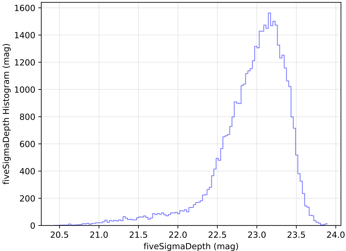
noroll_mjdp120_v3.4_10yrs Yr 1 z band: fiveSigmaDepth Histogram
