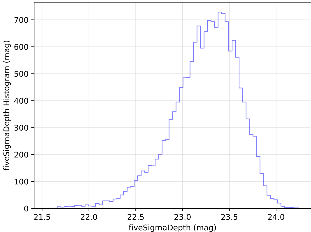
noroll_mjdp120_v3.4_10yrs Yr 1 u band: fiveSigmaDepth Histogram
