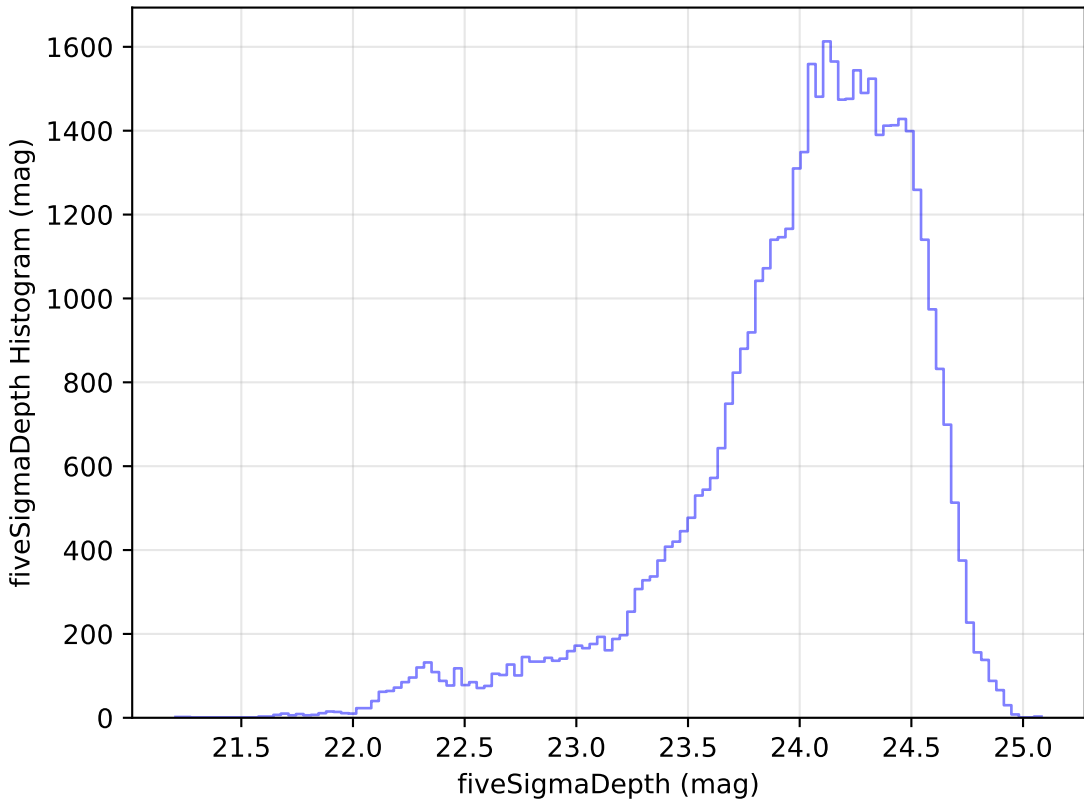
noroll_mjdp120_v3.4_10yrs Yr 1 r band: fiveSigmaDepth Histogram
