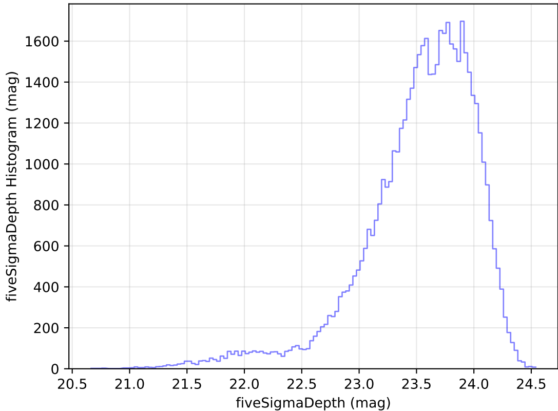
noroll_mjdp120_v3.4_10yrs Yr 1 i band: fiveSigmaDepth Histogram
