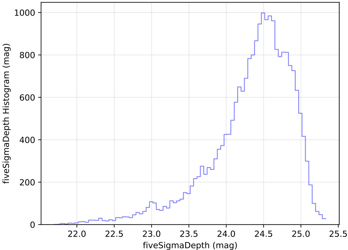
noroll_mjdp120_v3.4_10yrs Yr 1 g band: fiveSigmaDepth Histogram
