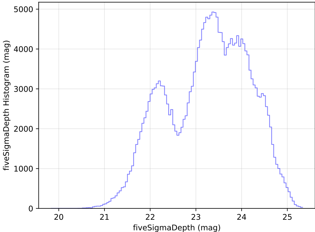
noroll_mjdp120_v3.4_10yrs Yr 1 all bands: fiveSigmaDepth Histogram
