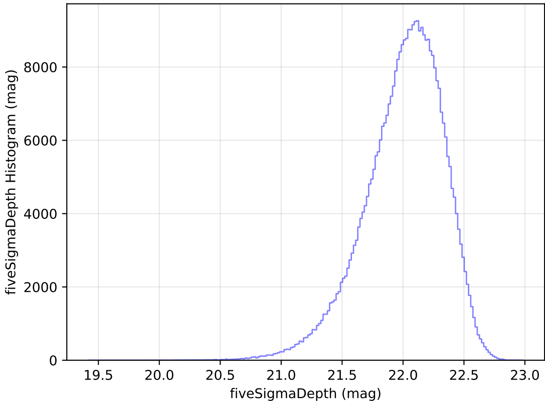
noroll_mjdp120_v3.4_10yrs WFD y band: fiveSigmaDepth Histogram
