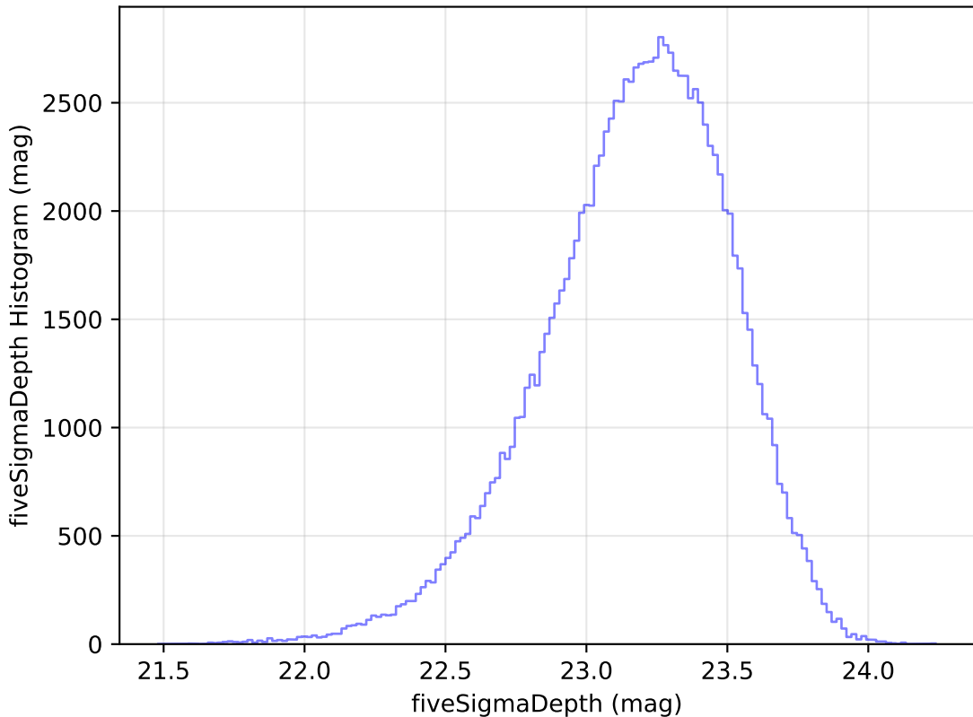
noroll_mjdp120_v3.4_10yrs WFD u band: fiveSigmaDepth Histogram
