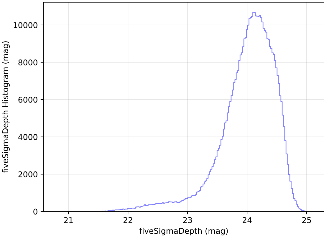
noroll_mjdp120_v3.4_10yrs WFD r band: fiveSigmaDepth Histogram
