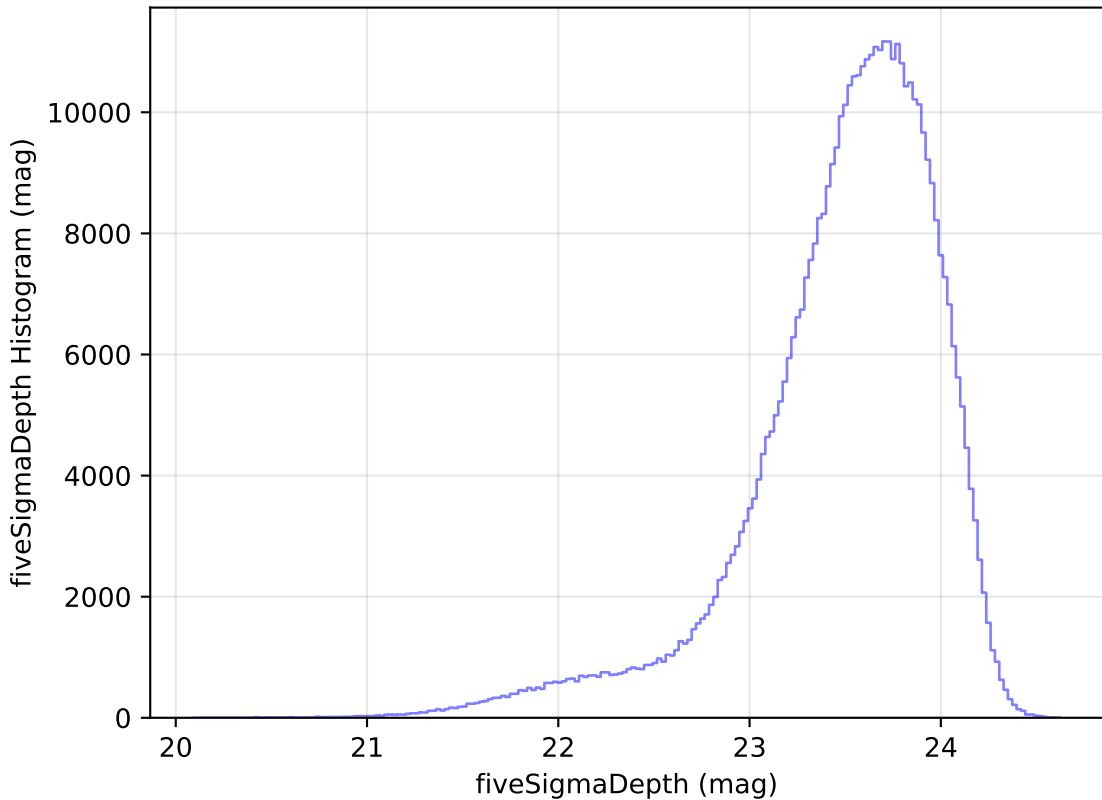
noroll_mjdp120_v3.4_10yrs WFD i band: fiveSigmaDepth Histogram
