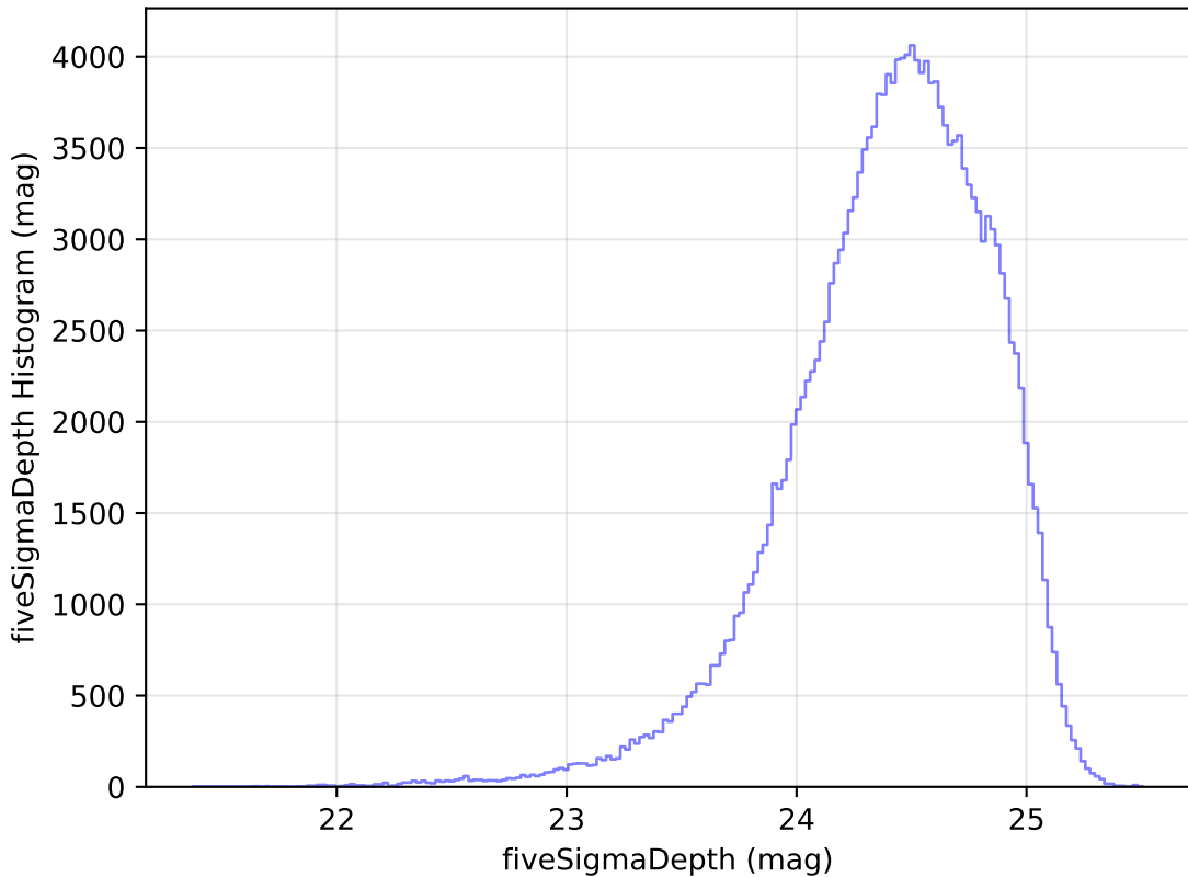
noroll_mjdp120_v3.4_10yrs WFD g band: fiveSigmaDepth Histogram
