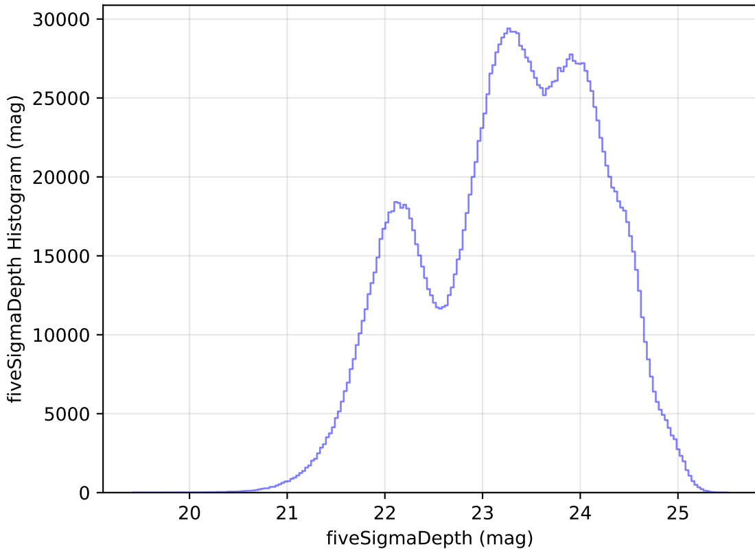
noroll_mjdp120_v3.4_10yrs WFD all bands: fiveSigmaDepth Histogram
