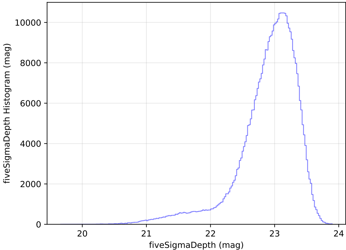
noroll_mjdp120_v3.4_10yrs All sky z band: fiveSigmaDepth Histogram
