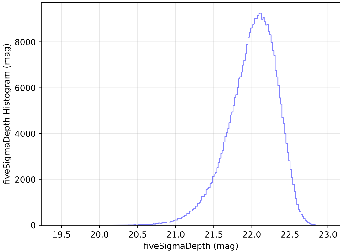
noroll_mjdp120_v3.4_10yrs All sky y band: fiveSigmaDepth Histogram
