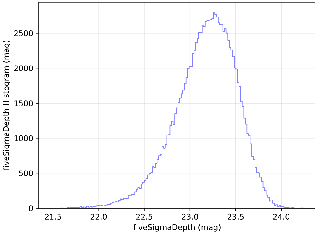
noroll_mjdp120_v3.4_10yrs All sky u band: fiveSigmaDepth Histogram
