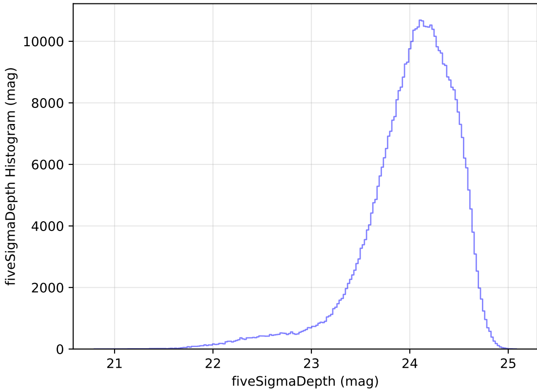
noroll_mjdp120_v3.4_10yrs All sky r band: fiveSigmaDepth Histogram
