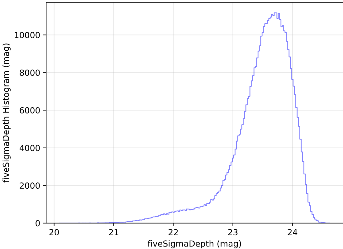
noroll_mjdp120_v3.4_10yrs All sky i band: fiveSigmaDepth Histogram
