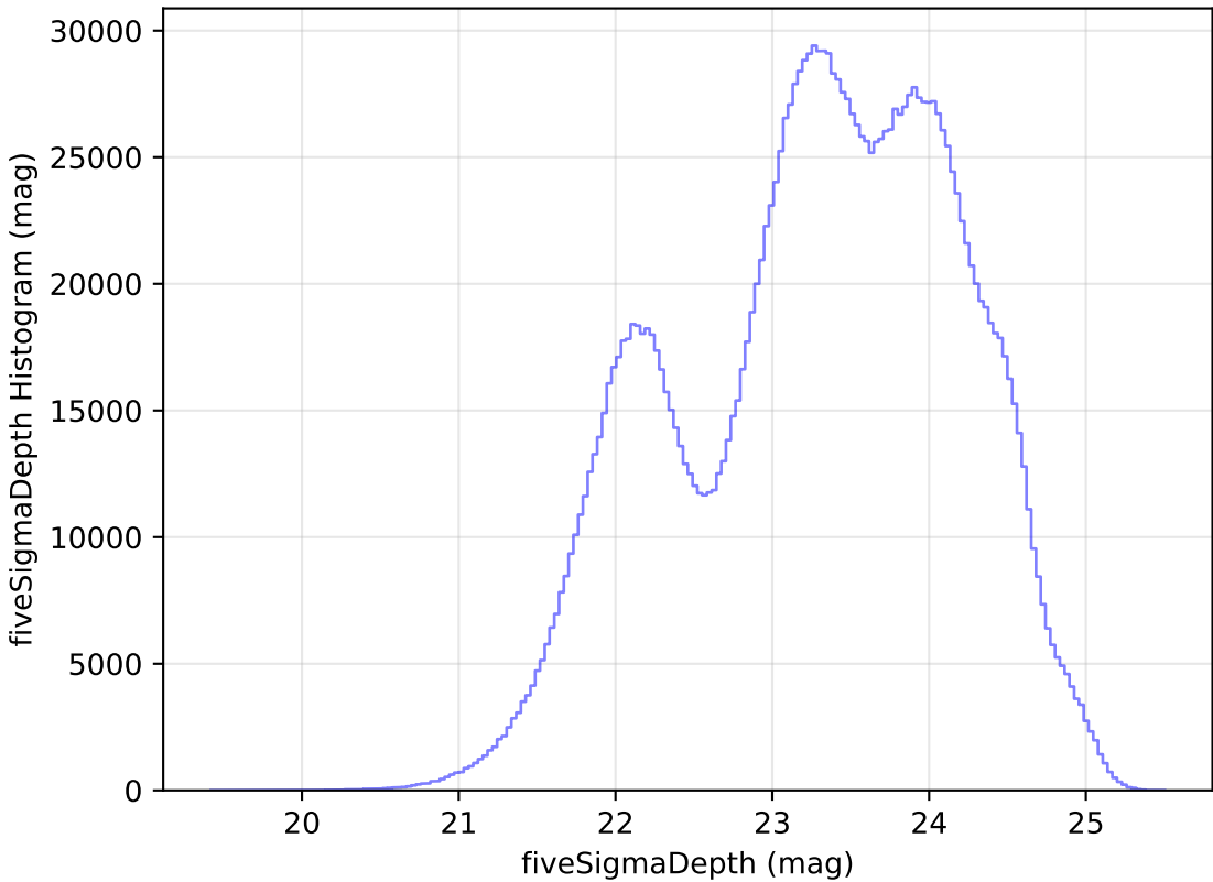
noroll_mjdp120_v3.4_10yrs All sky all bands: fiveSigmaDepth Histogram
