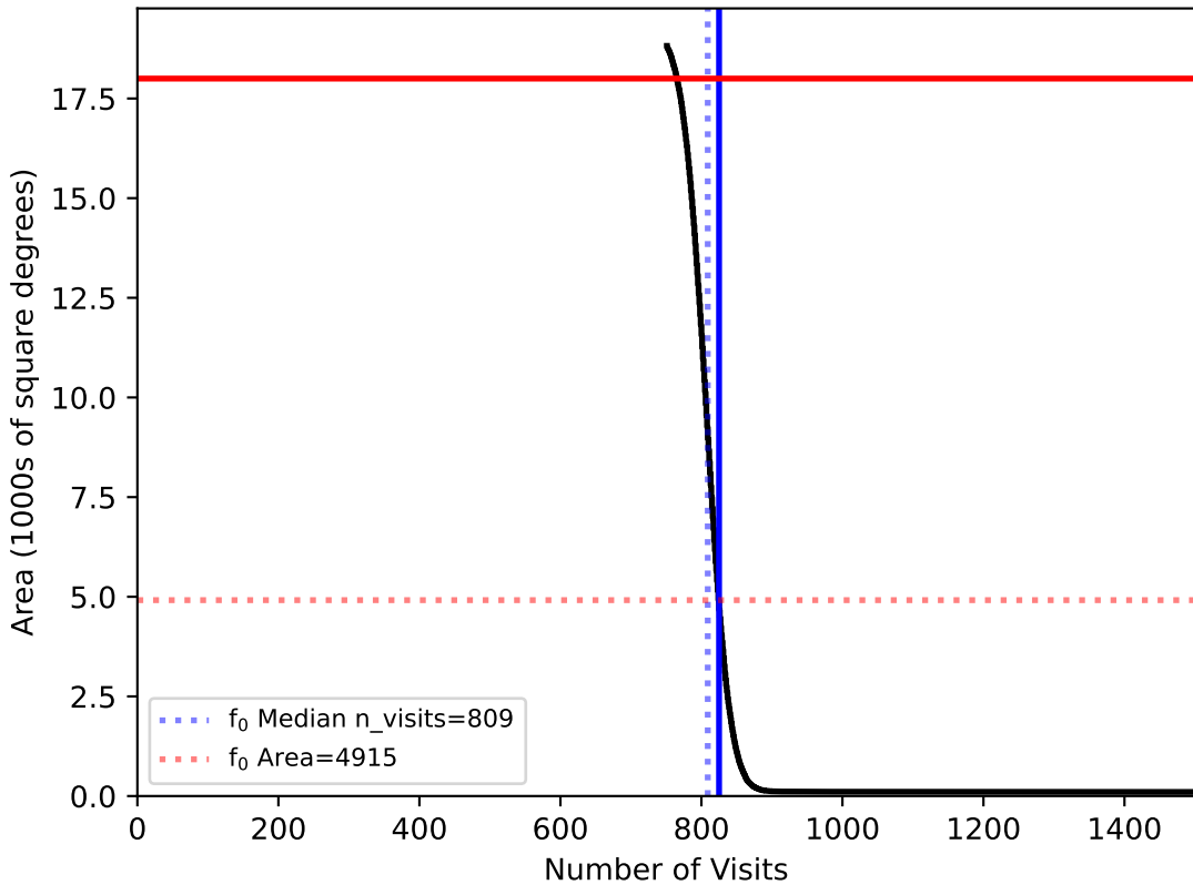
noroll_mjdp120_v3.4_10yrs WFD: f0
