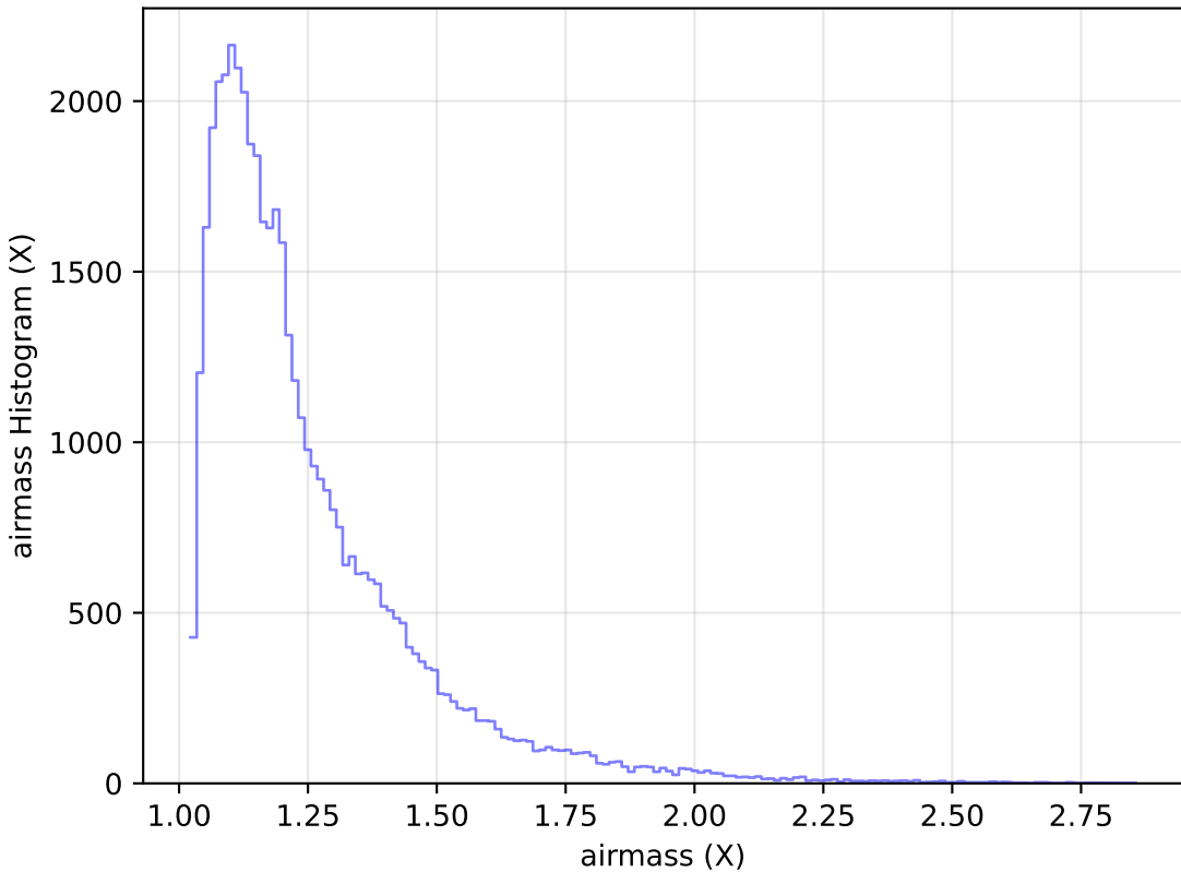
noroll_mjdp120_v3.4_10yrs Yr 1 y band: airmass Histogram
