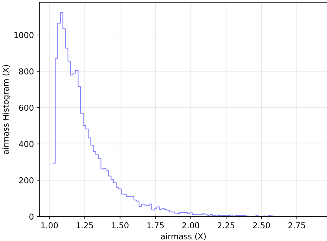
noroll_mjdp120_v3.4_10yrs Yr 1 u band: airmass Histogram
