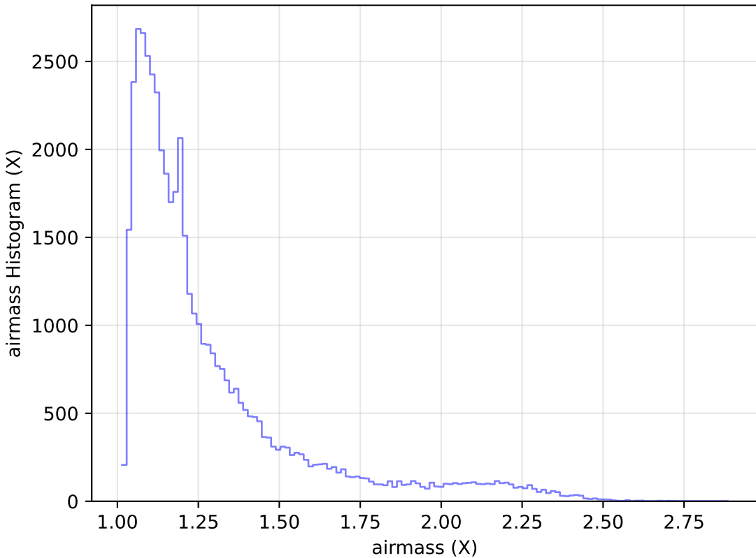
noroll_mjdp120_v3.4_10yrs Yr 1 r band: airmass Histogram
