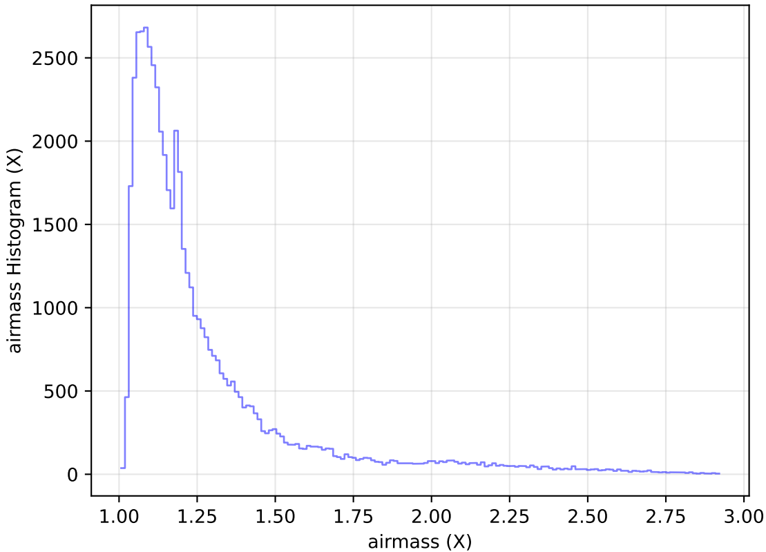
noroll_mjdp120_v3.4_10yrs Yr 1 i band: airmass Histogram
