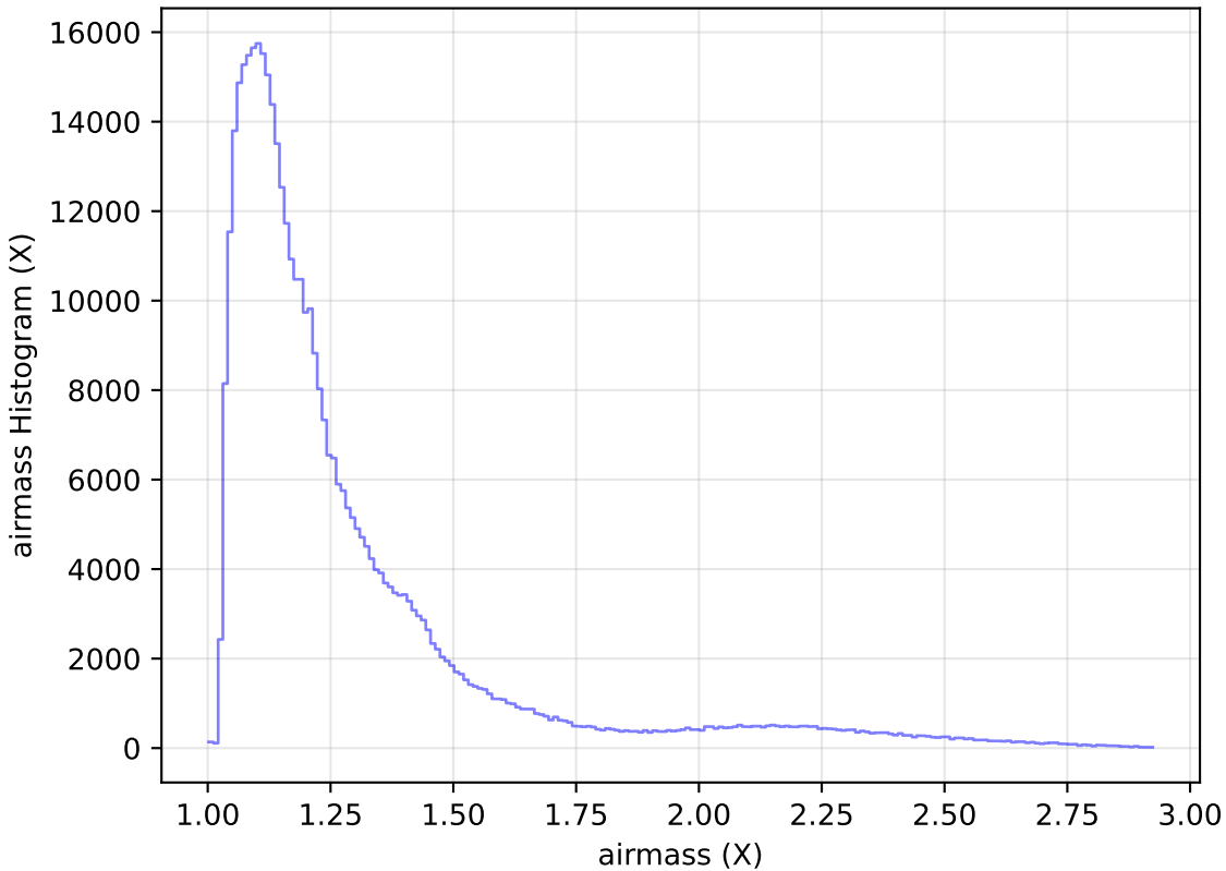
noroll_mjdp120_v3.4_10yrs WFD z band: airmass Histogram
